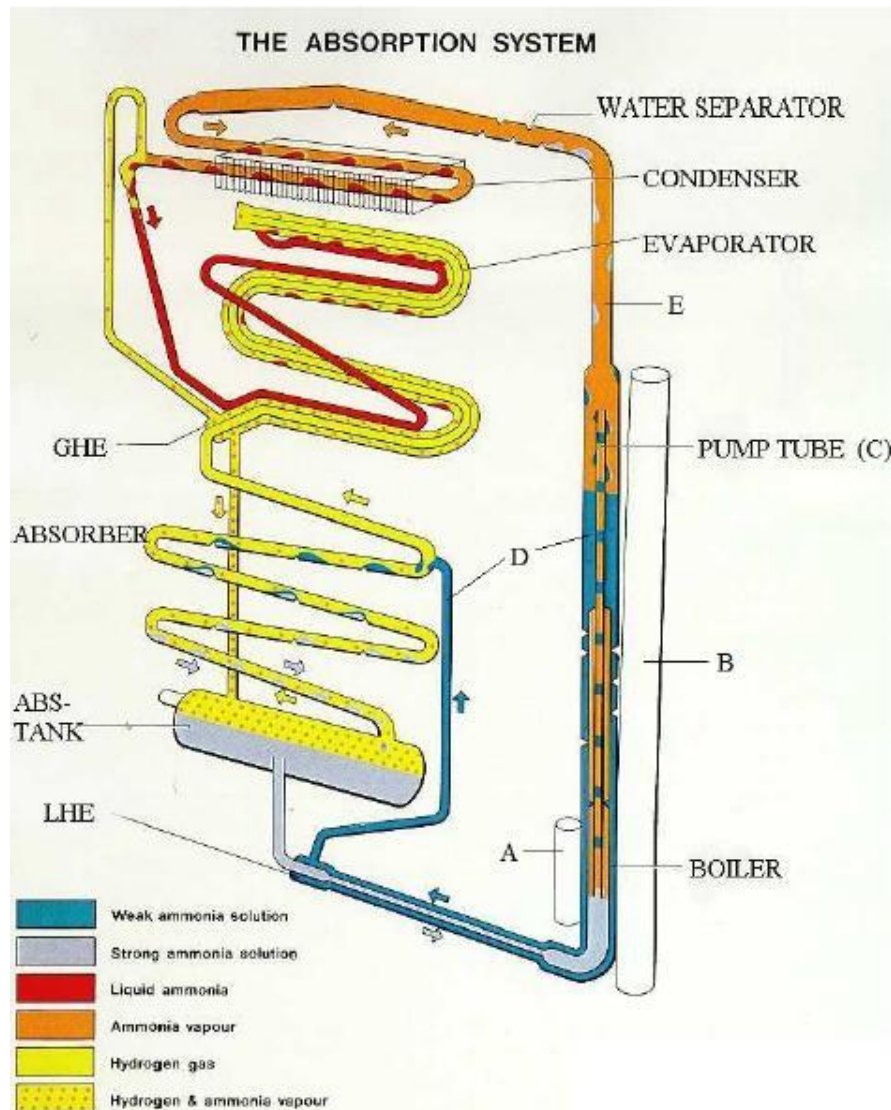
Figure 9-1: Scheme of the absorption cooling system
